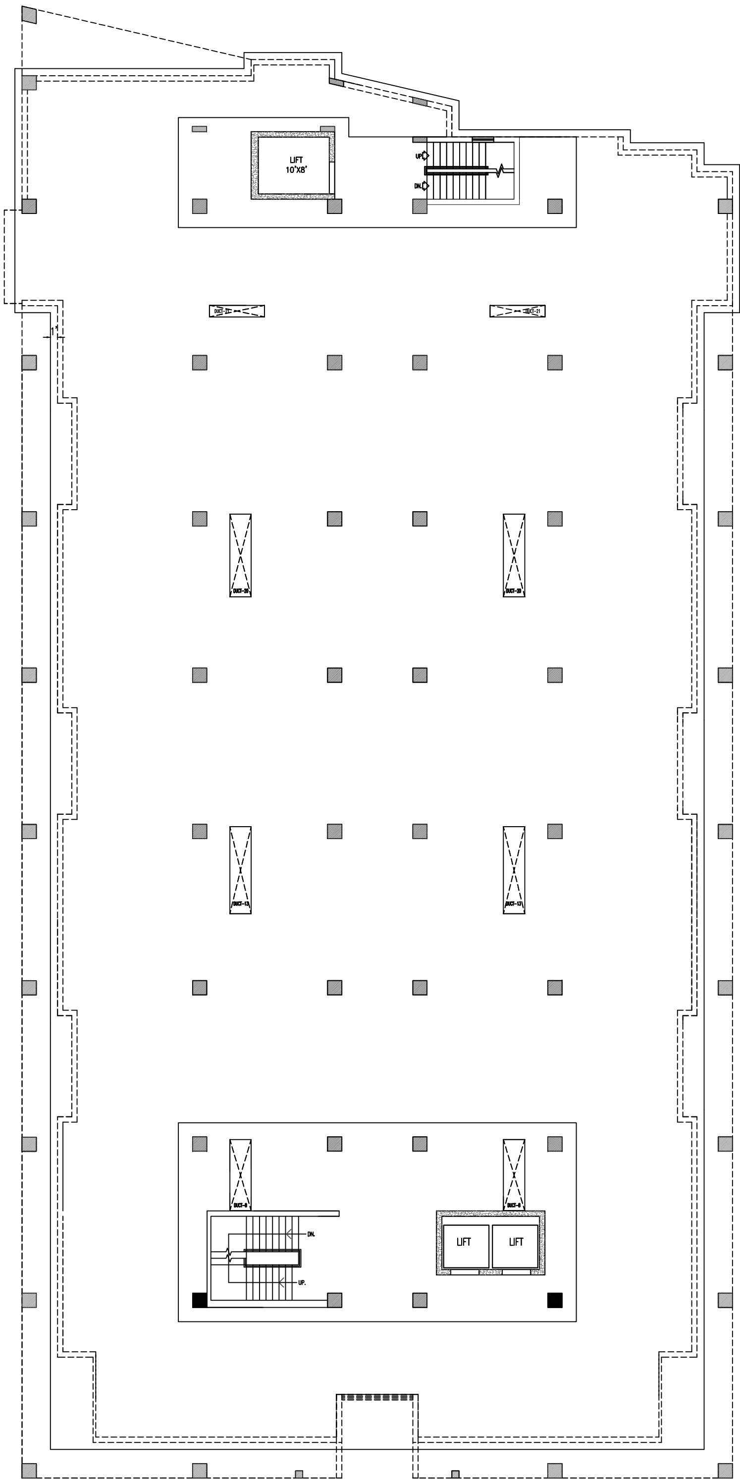
ROOF PLAN
