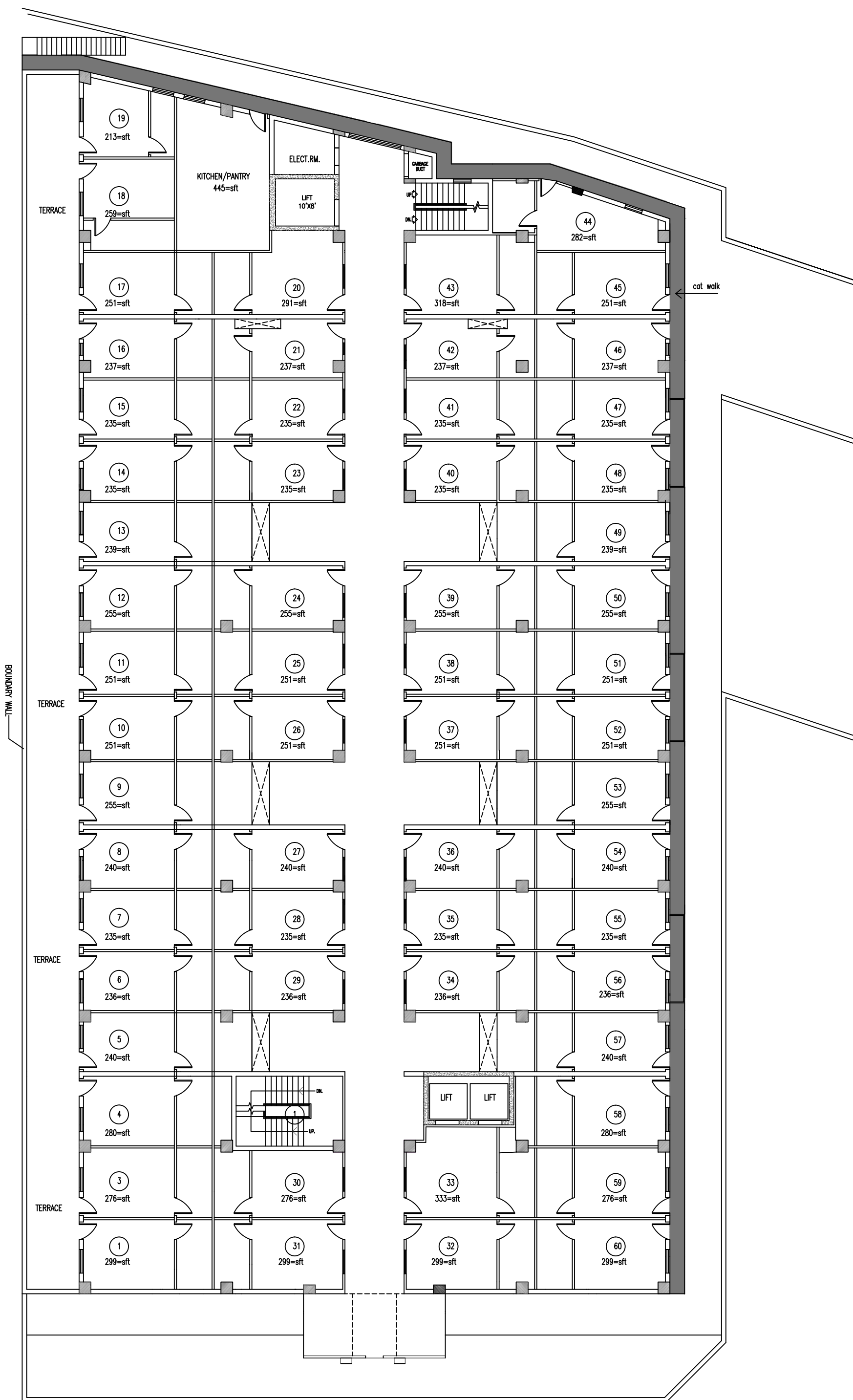
LOWER GROUND FLOOR PLAN(SERVANT QUARTERS)
